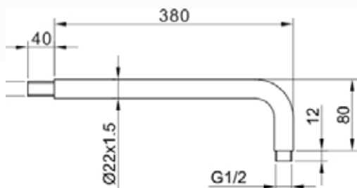
ST06SAK Mat zwart messing muurarm 380mm. Matt Black brass wall arm 380mm.
